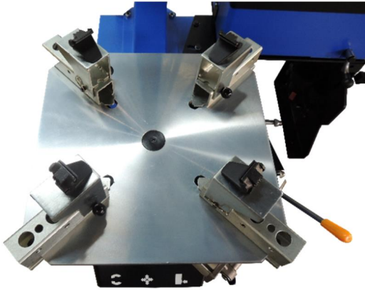
Unique Turntable Clamps Designed to Fit Motorcycle & ATV Rims with included Jaw Protectors
